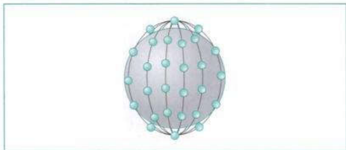
Figure 17.20 Iridium constellation
