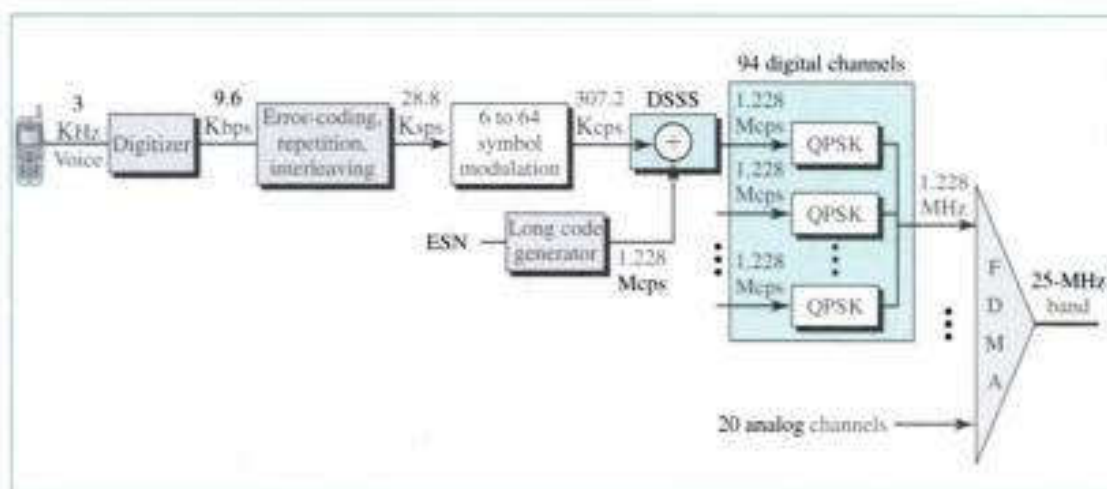
Figure 17.11 IS-95 reverse transmission
