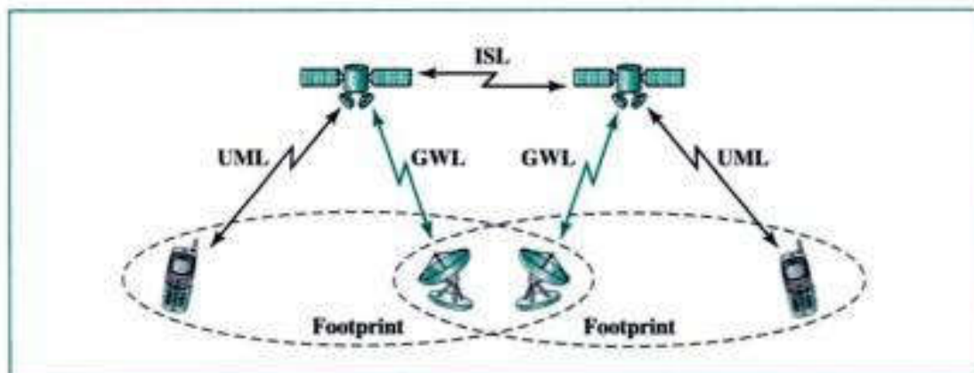
Figure 17.19 LEO satellite system
