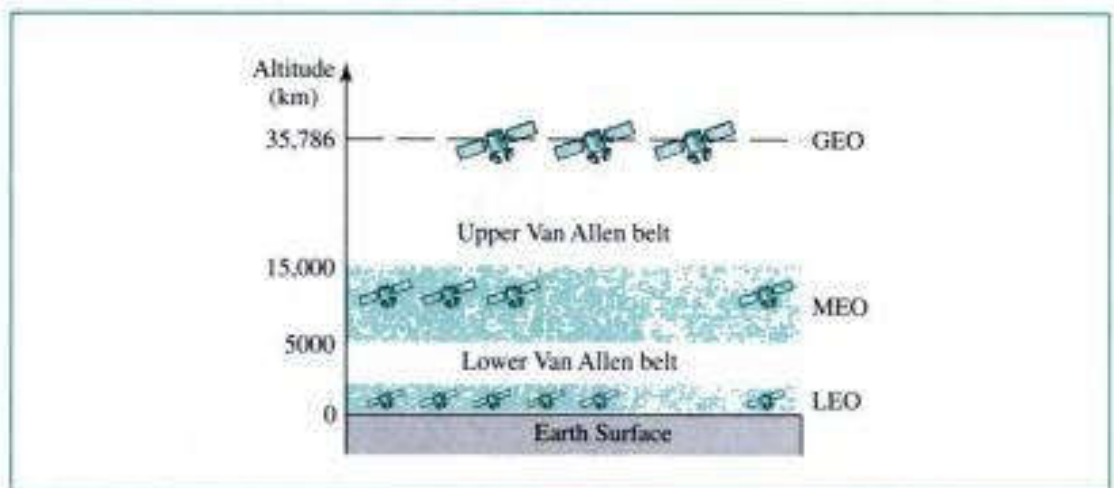
Figure 17.15 Satellite orbit altitudes
